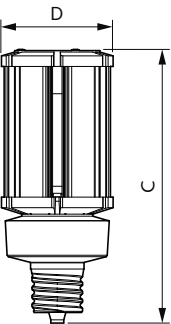
Corn lamp LED 36W EX39 840 CL Dim
